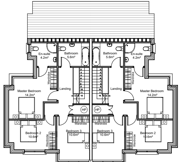
FLOOR AREA = 60.0m 2
